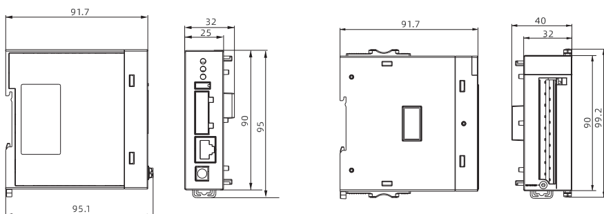
Left expansion module size diagram
