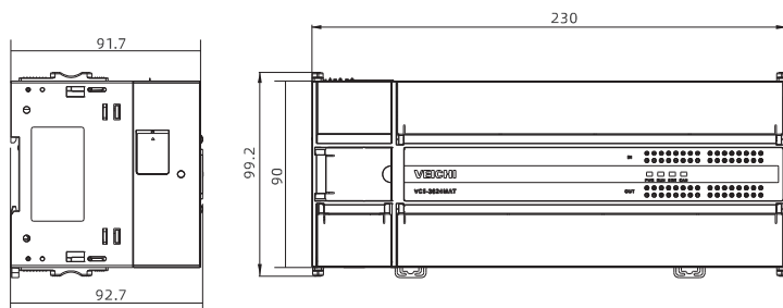
VC3/VC5 main module size diagram
