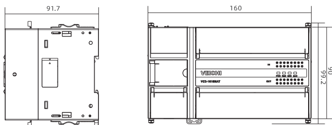
VC3/VC5 main module size drawing
