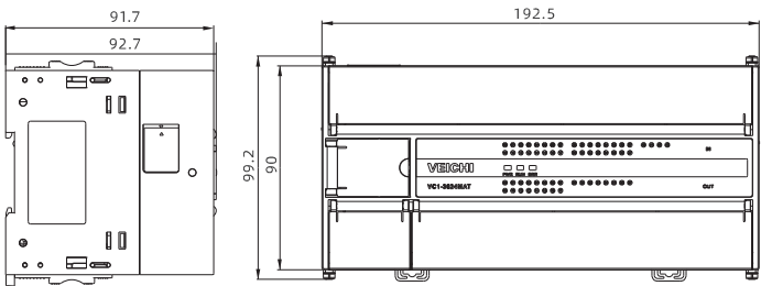
VC1 main module size diagram
